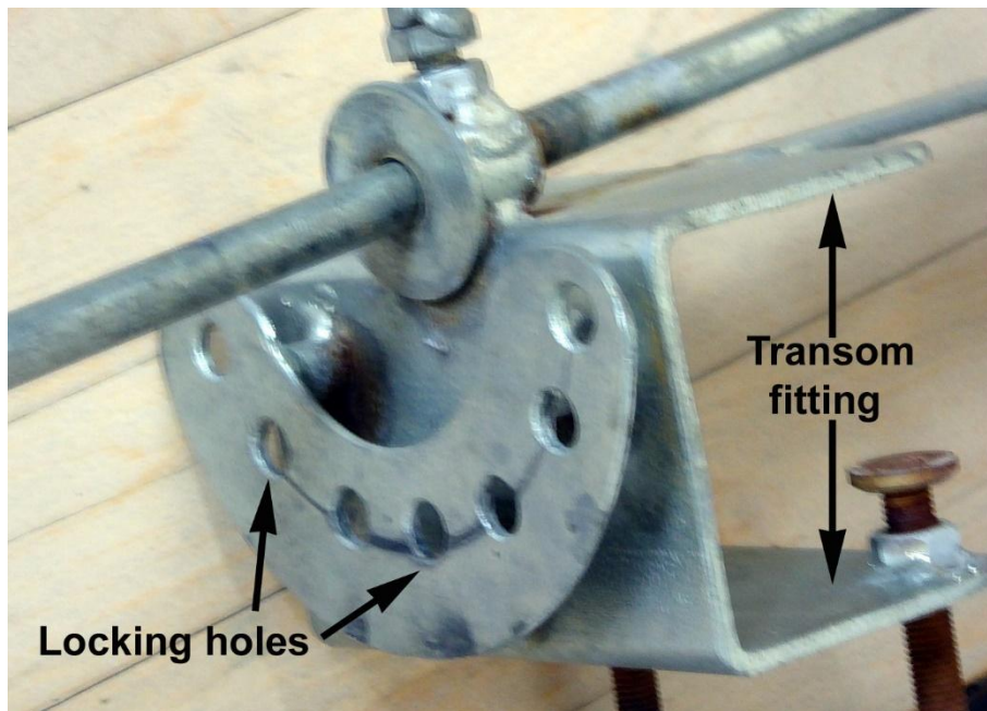
FIGURE 1. PETERS RUDDER. (note it has been hot dip galvanised which suggests that it is a commercial model. Google “fishing rudders” to find a load of info. on designs and how to use them.
